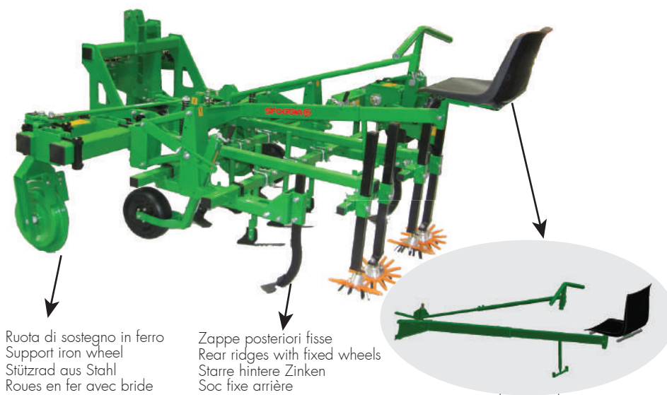
Kit guida manuale Manual steering device Manuelle Lenkung Kit guidage manuelle
